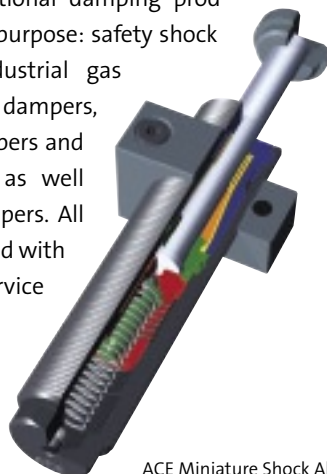
ACE Miniature Shock Absorber SC 2
